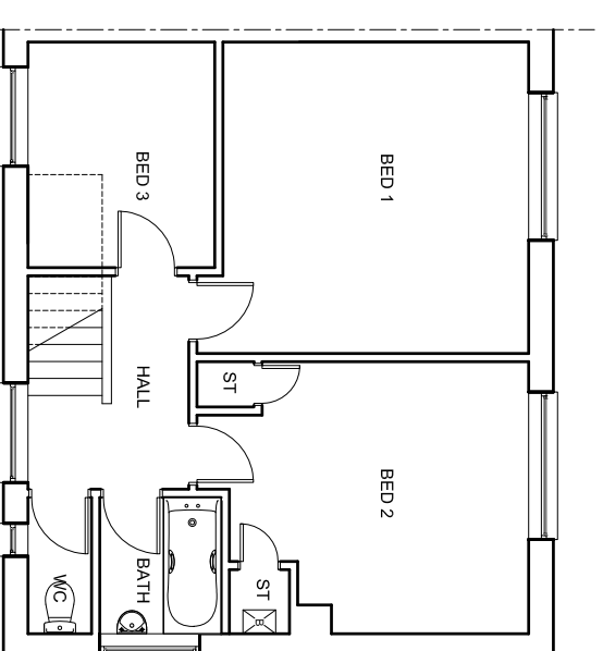
FF PLAN
